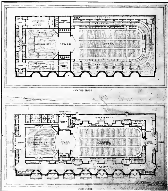
FIRST AND SECOND FLOOR PLANS, OAKLAND AUDITORIUM
